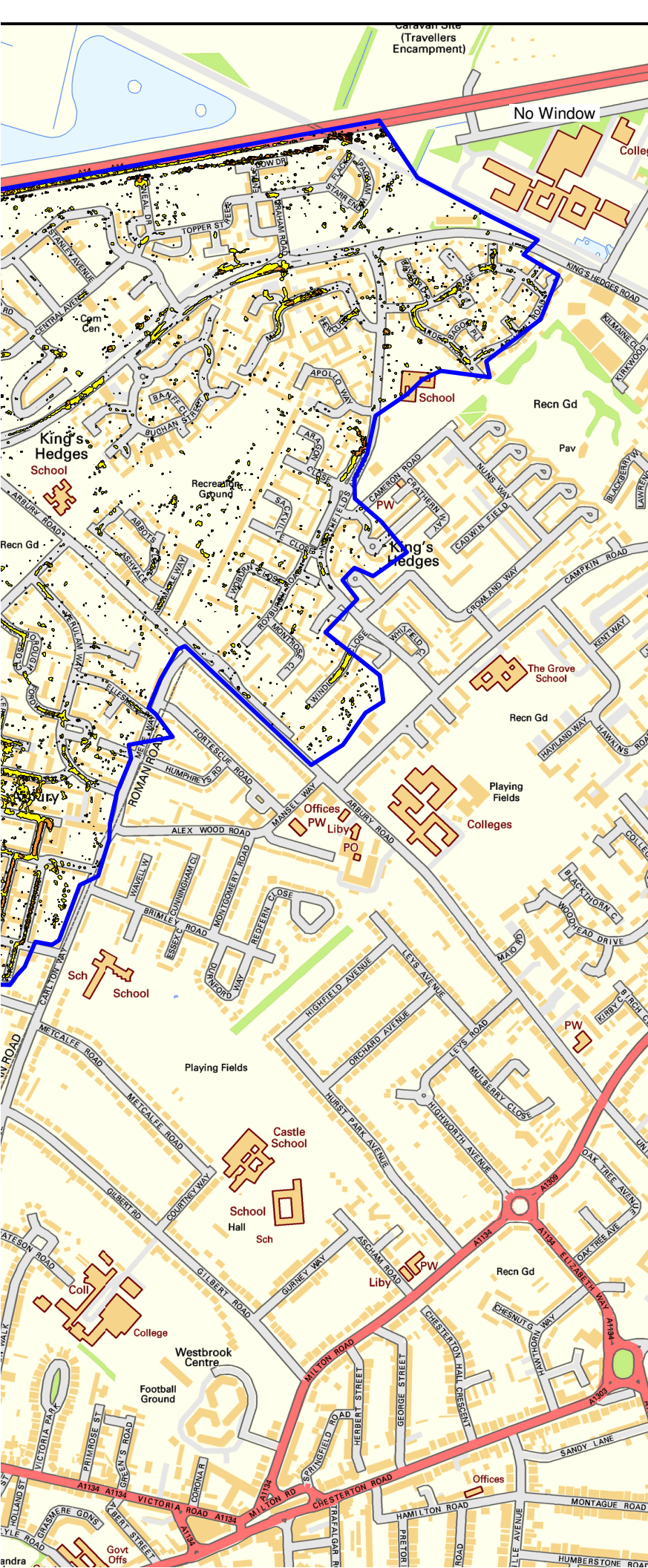
FIGURE F29 0.5% AEP "ENGINEERING OPTION C8" PLUVIAL MODELLING MAXIMUM VELOCITY - KING'S HEDGES AND ARBURY
